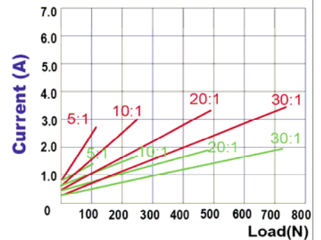
Current V.S. Load
